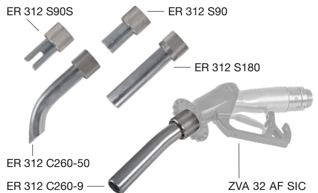
Exchangeable Spouts
